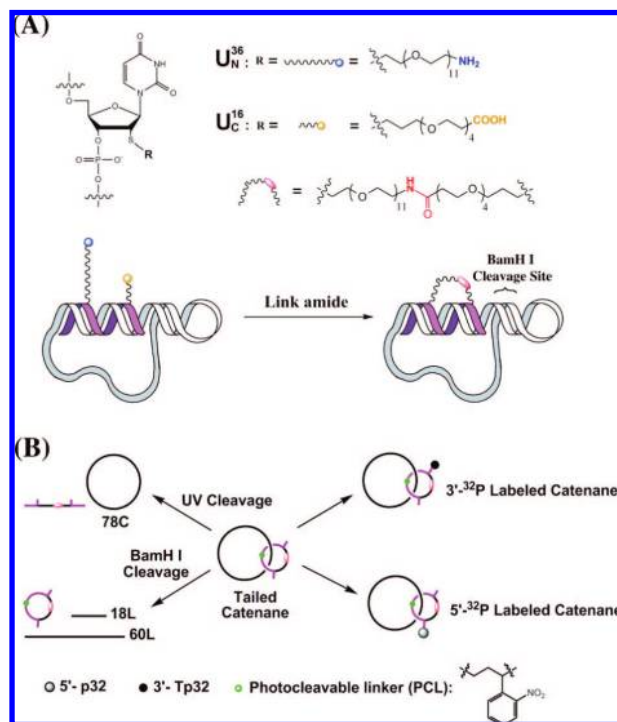
Figure 1. Schematic depiction of (A) templated synthesis of the tailed catenane, (B) cleavage, and labeling of the tailed catenane constructed from strand 4. The catenane stereoisomer is established by the antiparallel pairing of DNA before closure.
